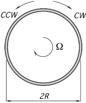
Fig. 8.13. Sagnac effect.
