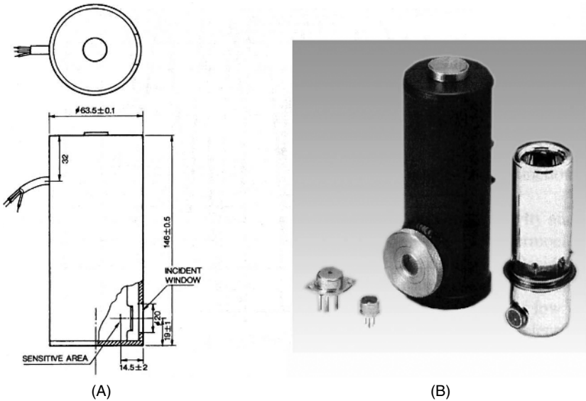
Fig. 14.17. Cryogenically cooled MCT quantum infrared detectors: (A) dimensional drawing of a Dewar type (in mm); (B) outside appearances of canned and Dewar detectors. (Courtesy of Hamamatsu Photonics K.K.)
