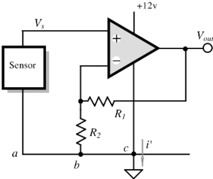
Fig. 5.54. Wrong connection of a ground terminal to a circuit (A); path of a supply current through the ground conductors (B).
