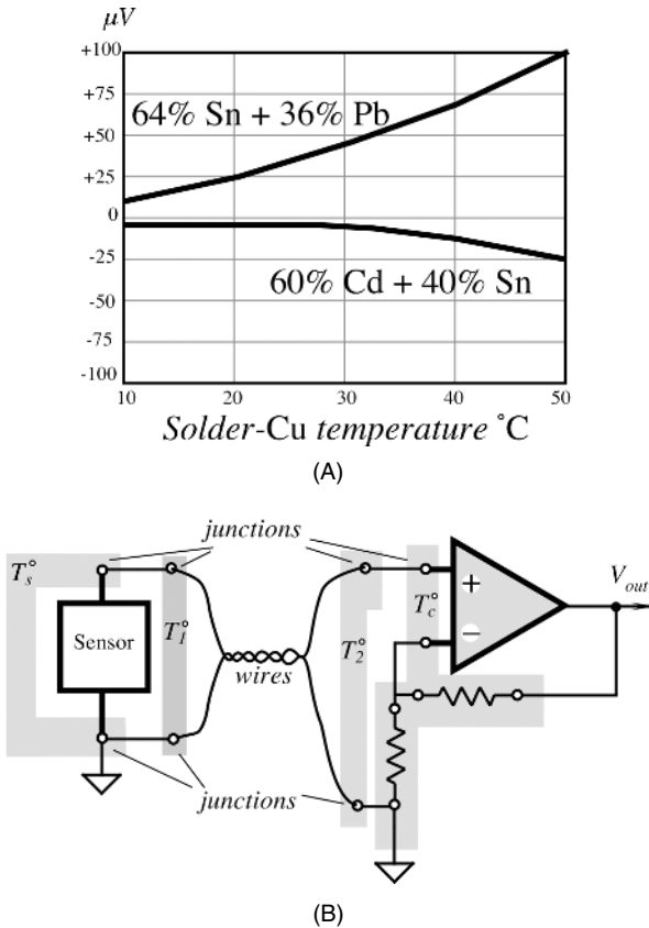
Fig. 5.56. (A) Seebeck e.m.f. developed by solder–copper joints (Adapted from Ref. [17]); (B) Maintaining joints at the same temperature reduces Seebeck noise.
