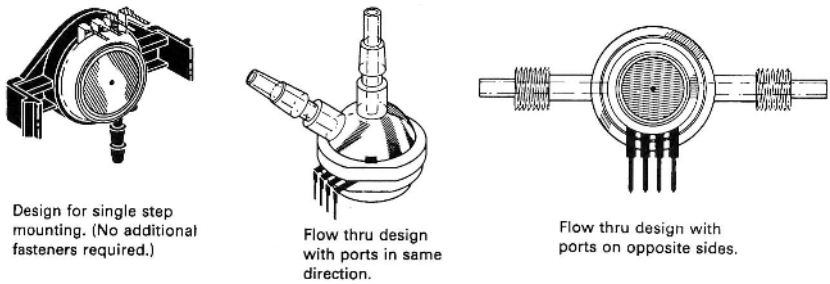
Fig. 10.8. Examples of differential pressure packaging. (Copyright Motorola, Inc. Used with permission.)
