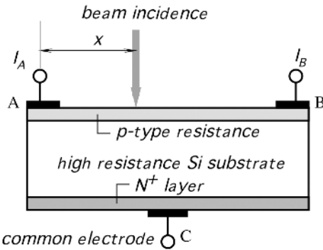
Fig. 7.36. Design of a one-dimensional PSD.
