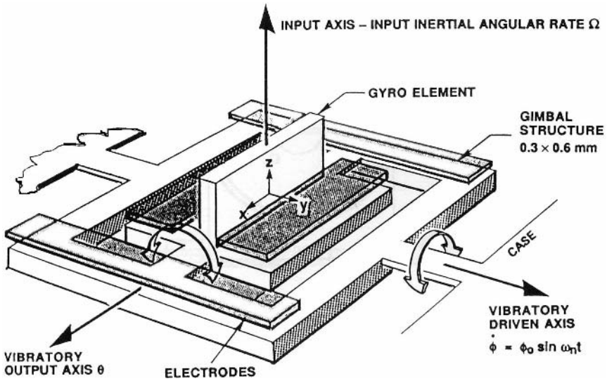
Fig. 8.12. Vibratory rate gyro concept. (From Ref. [7].)
