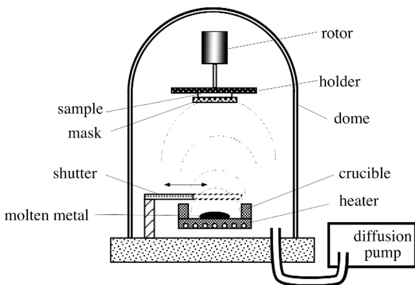
Fig. 18.5. Deposition of a thin metal film in a vacuum chamber.
