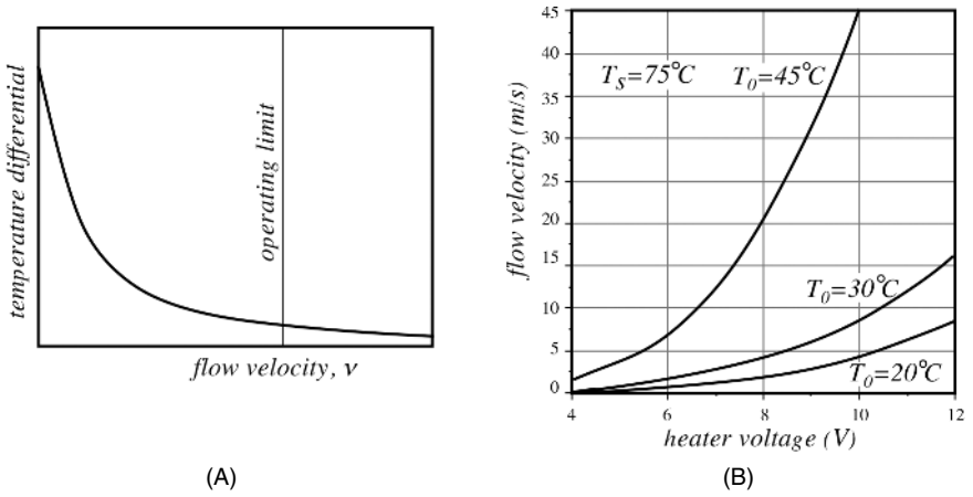
Fig. 11.5. Transfer function of a thermoelement (A) and calibration curves for a self-heating sensor in a thermoelement for three different levels of heat (B).
