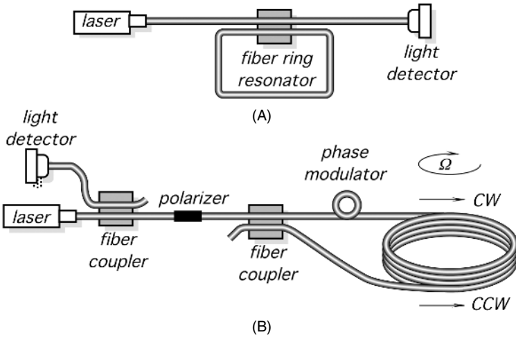
Fig. 8.14. (A) Fiber-optic ring resonator; (B) fiber-optic analog coil gyro. (Adapted from Ref. [9].)
