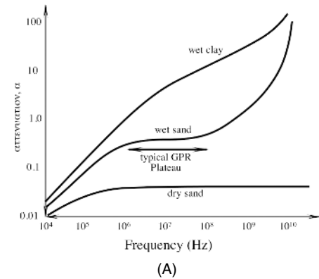
Fig. 7.44. (A) Attenuation of radio waves in different materials. Attenuation varies with excitation frequency and type of material. At low frequencies ( < 1 MHz), attenuation is primarily controlled by dc conductivity. At high frequencies ( > 1000 MHz), water is a strong energy absorber. (B) When attenuation limits exploration depth, power must increase exponentially with depth.
