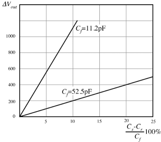
Fig. 5.33. Transfer function of a capacitance-to-voltage converter for two values of integrating capacitor. (Adapted from Ref. [6])
