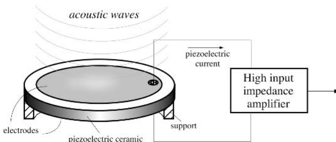
Fig. 12.4. Piezoelectric microphone.
