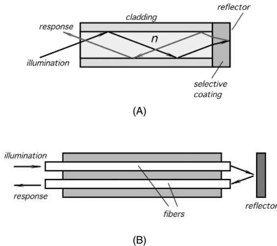
Fig. 4.17. (A) Single- and (B) dual-fiber-optic sensors.
