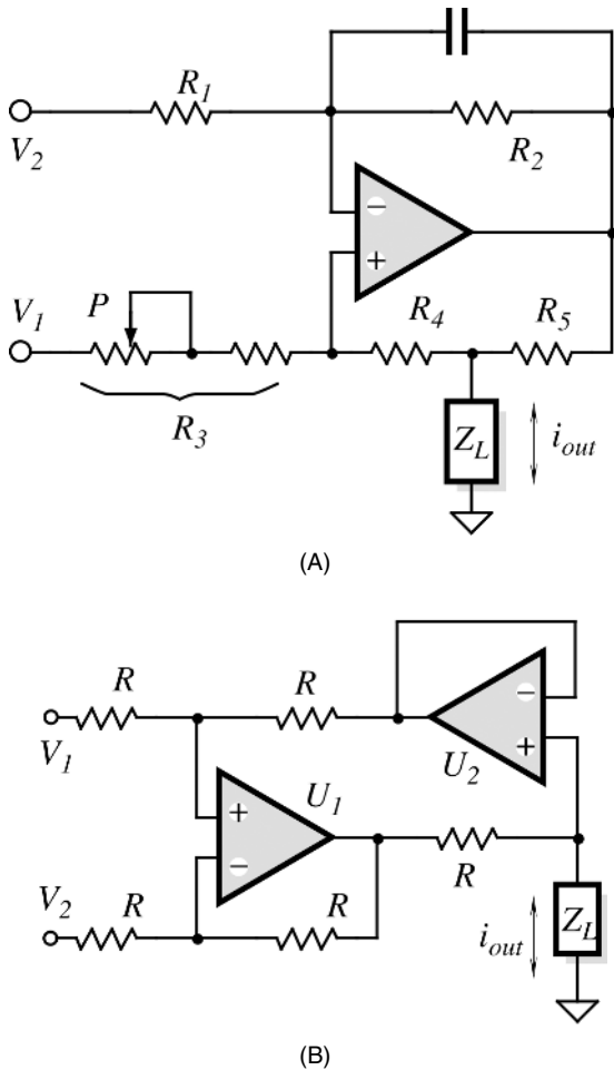
Fig. 5.15. Current generators with ground-referenced loads: (A) Howland current pump; (B) current pump with two OPAMs.
