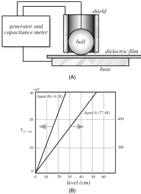
Fig. 7.48. Dry dielectric film capacitive sensor (A) and shape of transfer function (B). (Adapted from Ref. [16].)
