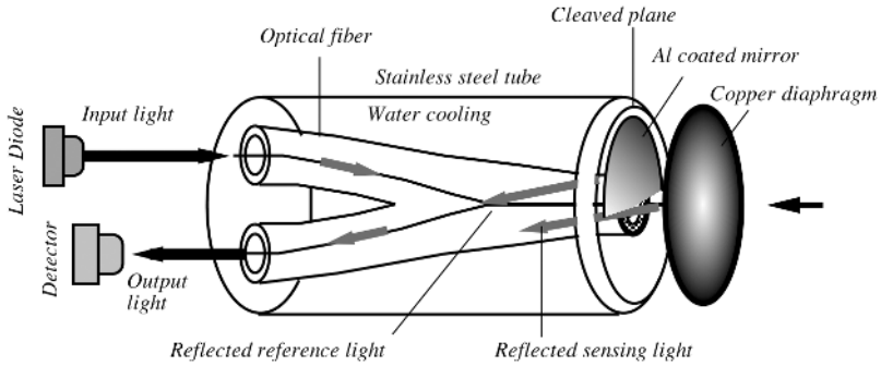
Fig. 12.2. Fiber-optic interferometric microphone. Movement of the copper diaphragm is converted into light intensity in the detector.
