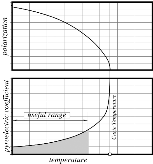
Fig. 3.28. Polarization of a pyroelectric crystal. The sensor must be stored and operated below the Curie temperature.
