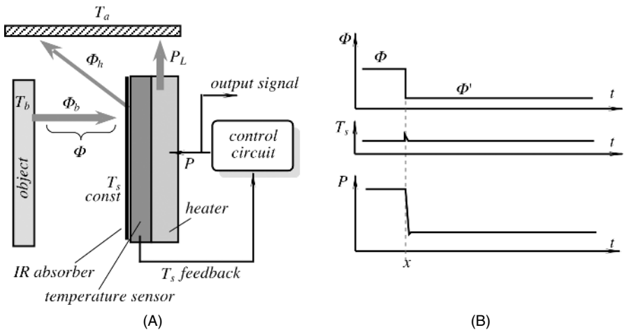
Fig. 14.28. The AFIR element radiates thermal flux \Phi_h toward its housing and absorbs flux \Phi_b from the object (A); timing diagrams for radiative flux, surface temperature, and supplied power (B).
