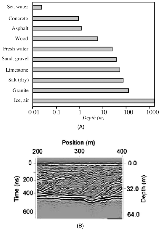
Fig. 7.45. (A) Maximum depth for various materials; (B) graphic presentation of measured bedding in wet sand deposits. (Courtesy of Sensors & Software, Inc., Canada, www.senssoft.ca .)
