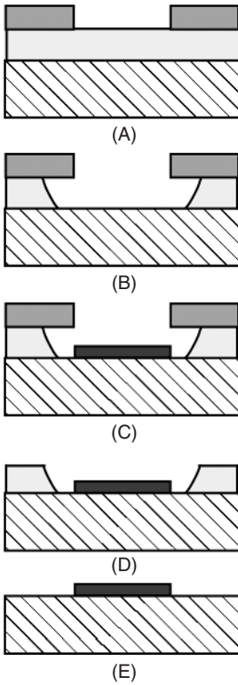
Fig. 18.16. Lift-off technique.
