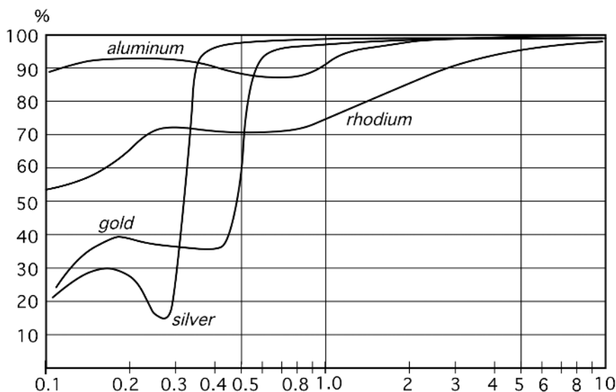
Fig. 4.10. Spectral reflectances of some mirror coatings.
