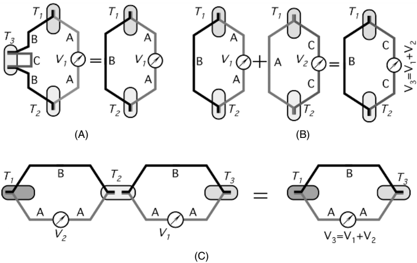
Fig. 16.15. Illustrations for the Laws of Thermocouples.
