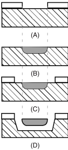
Fig. 18.13. Etching around the boron-doped silicon.
