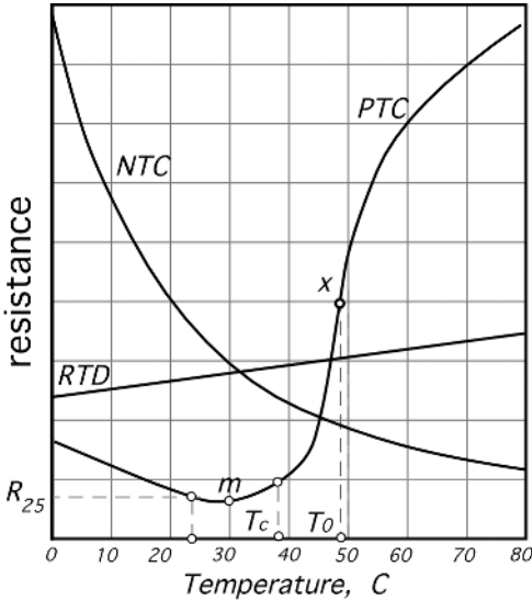
Fig. 16.12. Transfer functions of PTC and NTC thermistors as compared with an RTD.
