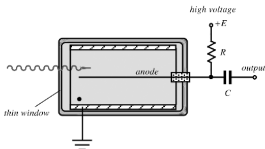
Fig. 15.5. Circuit of a Geiger-Müller counter. The symbol • indicates gas.
