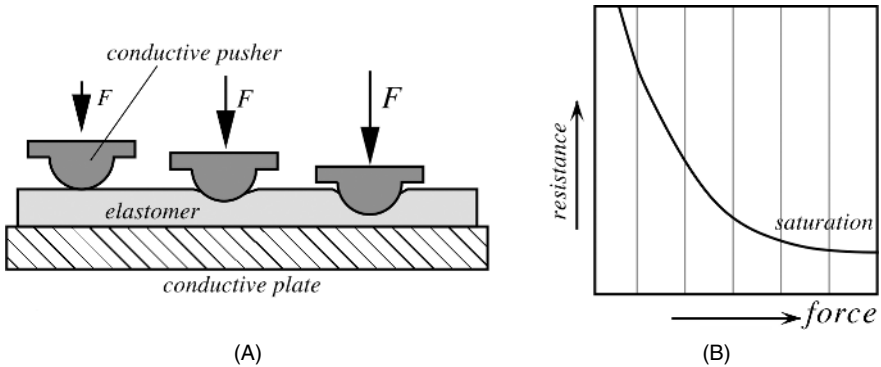
Fig. 9.8. FSR tactile sensor: (A) through-thickness application with an elastomer; (B) transfer function.
