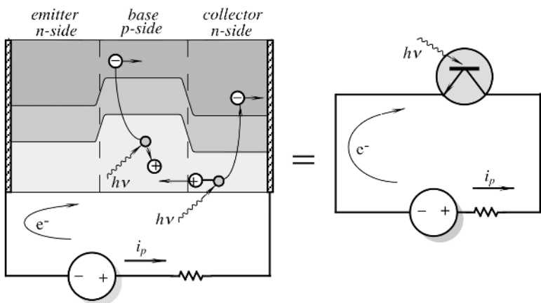
Fig. 14.11. Energy bands in a phototransistor.
