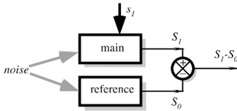
Fig. 5.47. Differential technique.
