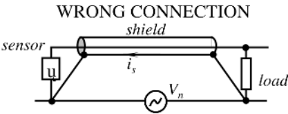
Fig. 5.50. Cable shield is erroneously grounded at both ends.
