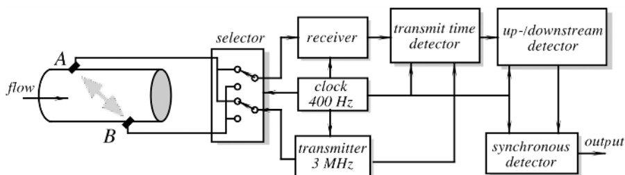
Fig. 11.8. Block diagram of an ultrasonic flowmeter with alternating transmitter and receiver.
