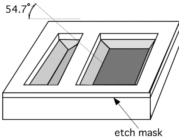
Fig. 18.10. Simple structures etched by KOH.
