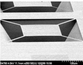
Fig. 14.26. Platinum-film bolometer: (A) glass membrane over the etched cavity; (B) array of bolometers.
