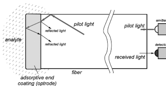
Fig. 17.13. Fiber-optic gas sensor.
