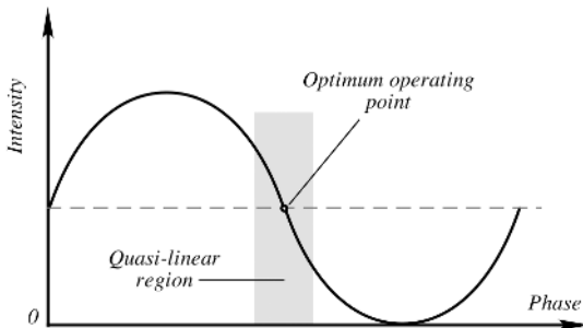
Fig. 12.3. Intensity plot as function of a reflected light phase.
